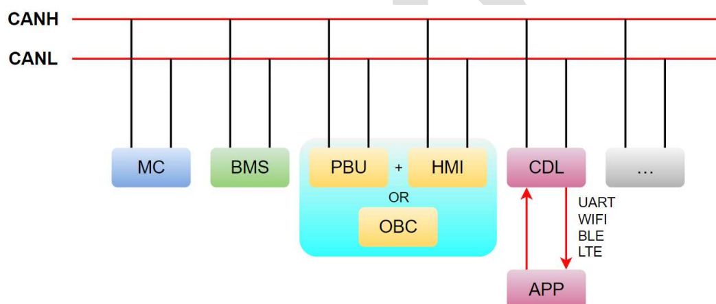
Figure1 Schematic diagram of system communication interface
